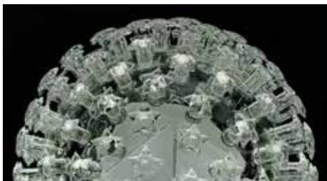
Detail from Papilloma virus
