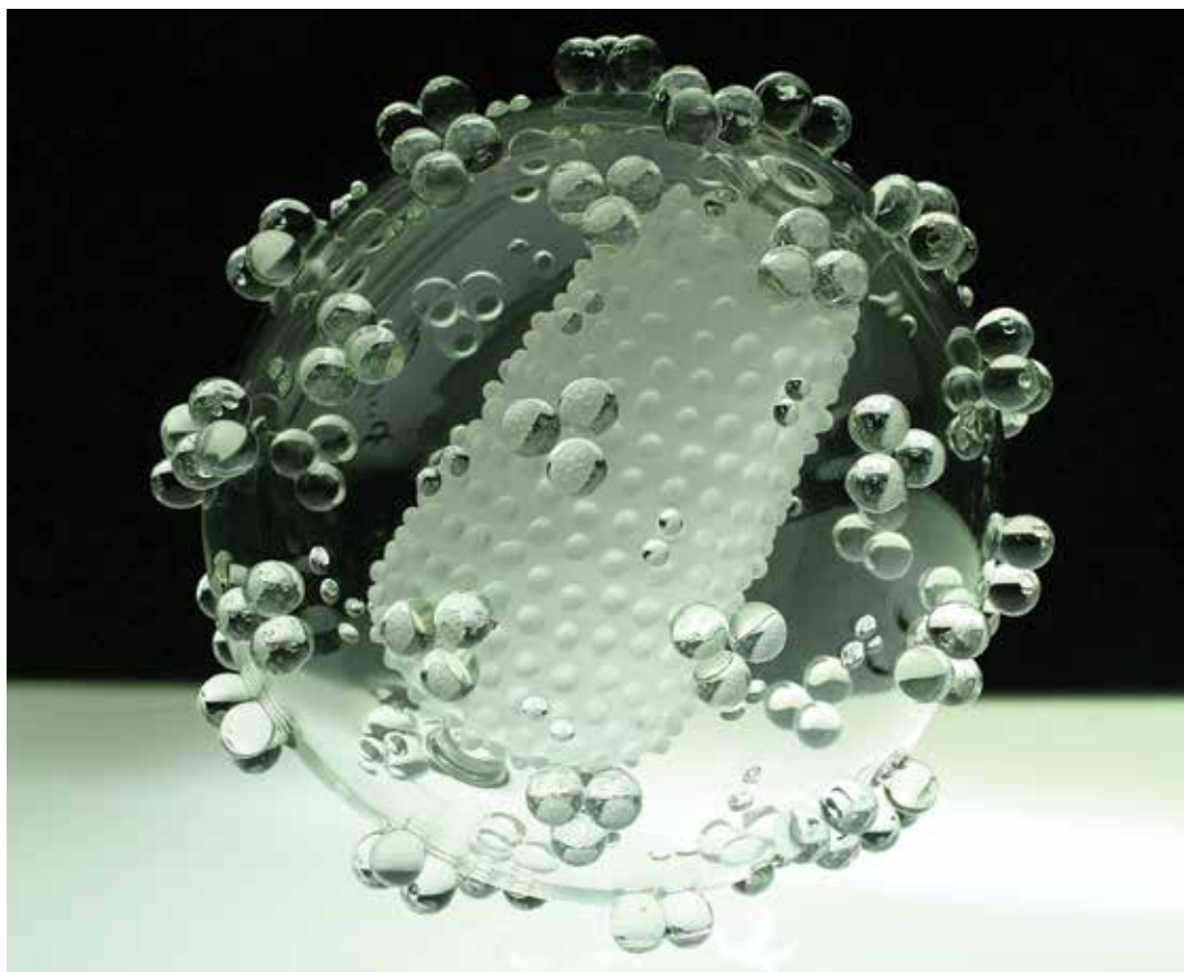
HIV, lipid membrane, glycoprotein, and capsid
